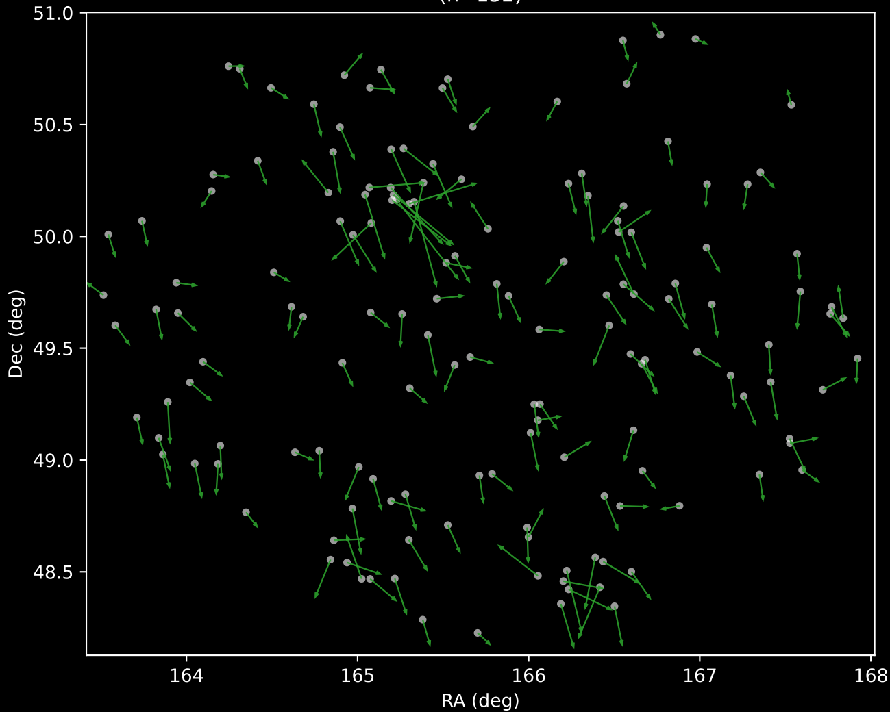
APOGEE DR17 Cluster 4 Proper Motion Vectors (n=152)
