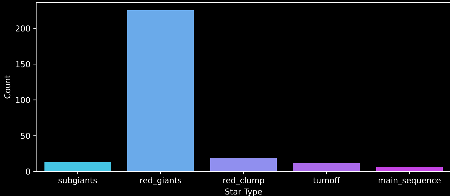
APOGEE DR17 Field: [154+00] Count plot of Star Type
