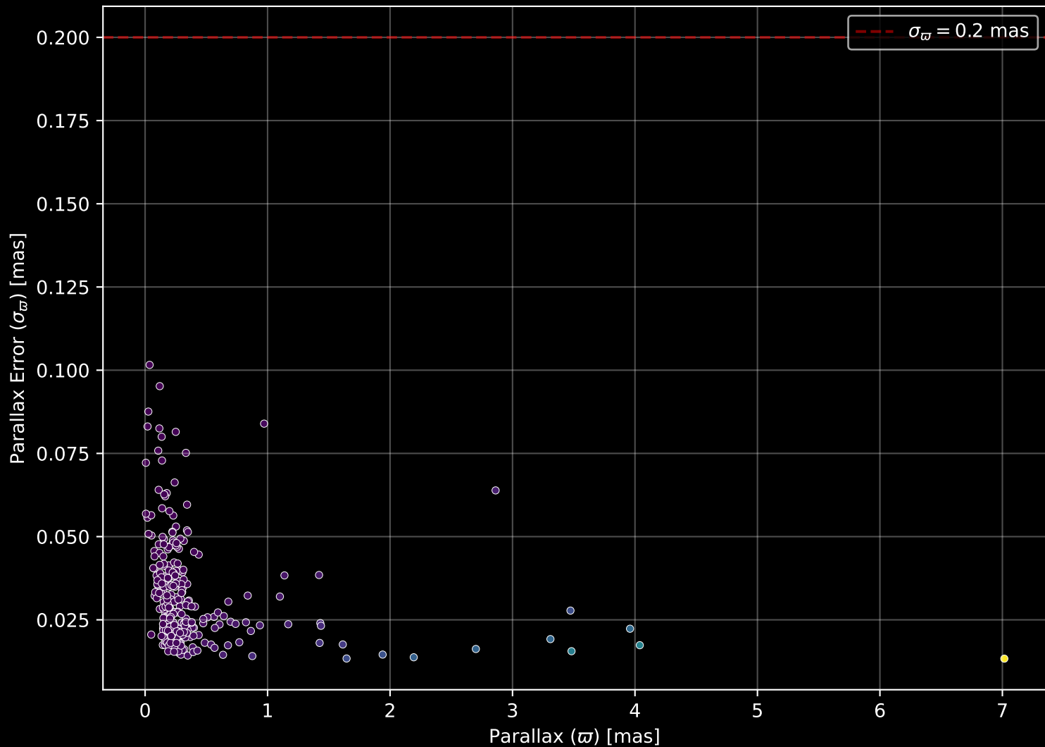
APOGEE DR17 Field: [154+00] Parallax Quality (n= 274)
