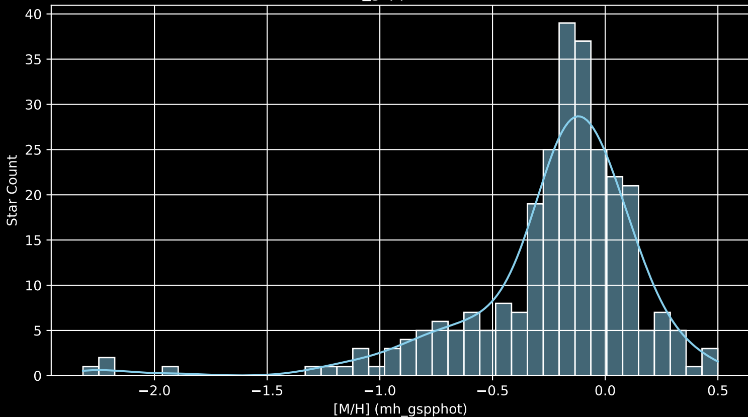
APOGEE DR17 Field: [154+00 [M/H] (mh_gspphot) (n= 270)
