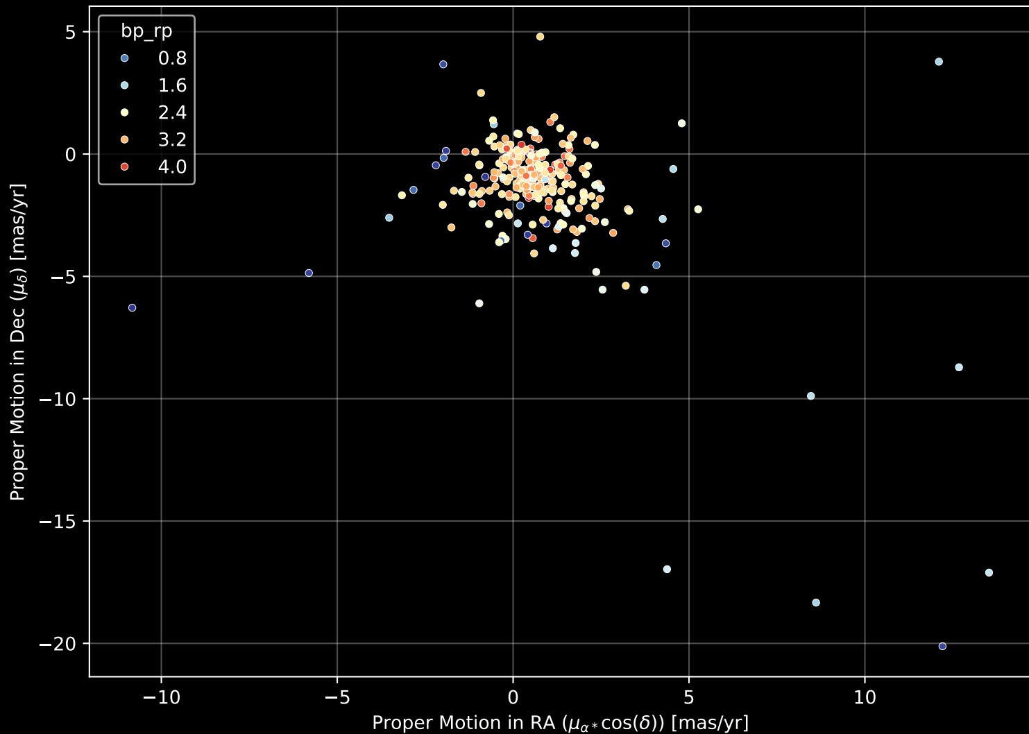
APOGEE DR17 Field: [154+00] Proper Motion Diagram (n= 274)
