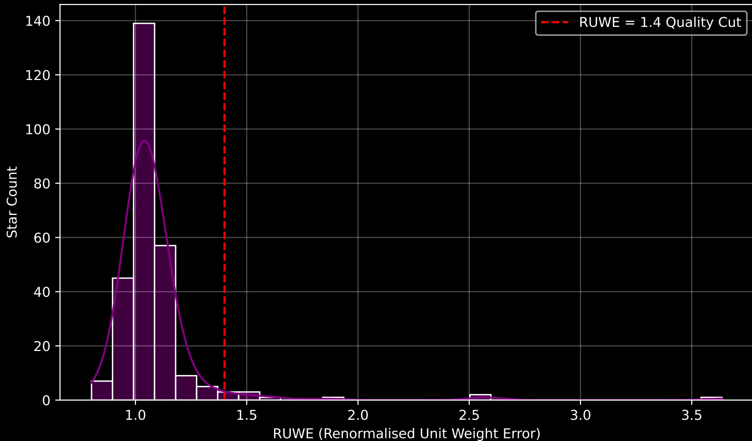
GAPOGEE DR17 Field [154+00] RUWE Distribution (n= 273)
